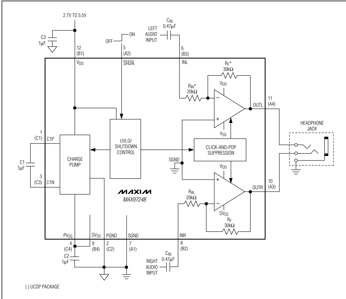
Functional Diagram/Typical Operating Circuits (continued)
